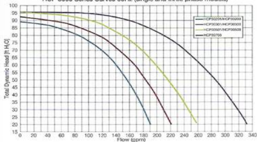
HCP 3000 Series Curves 60Hz (single and three phase models)
