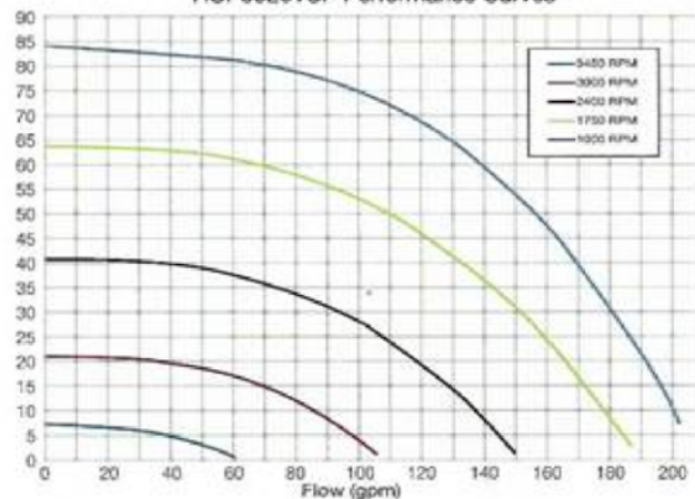
HCP3020VSP Performance Curves
